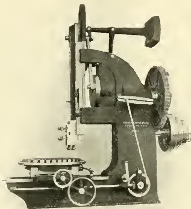
22-INCH CRANK SLOTTING MACHINE. Niles-Bement-Pond Co.
